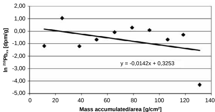
FIGURE 3. The excess {}^{210}\text{Pb} activity plotted against the mass accumulated per area in the sediments profile sampled at the Amazonas River mouth
